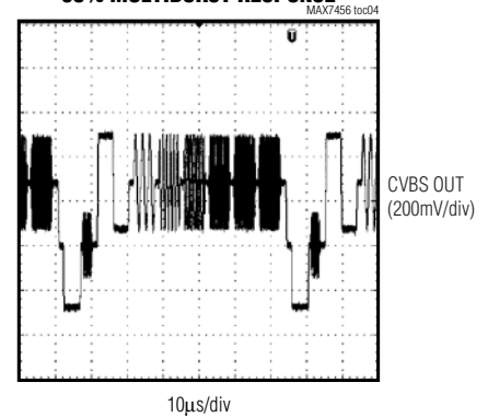
60% MULTIBURST RESPONSE
