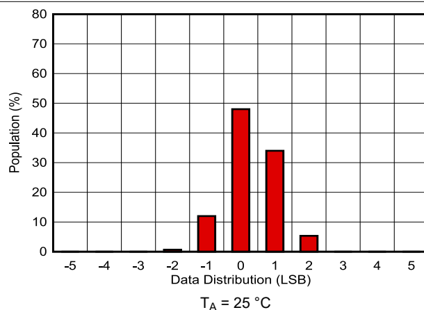
Figure 7-17. Data Distribution With 2-ms Conversion Time and Averaging On
