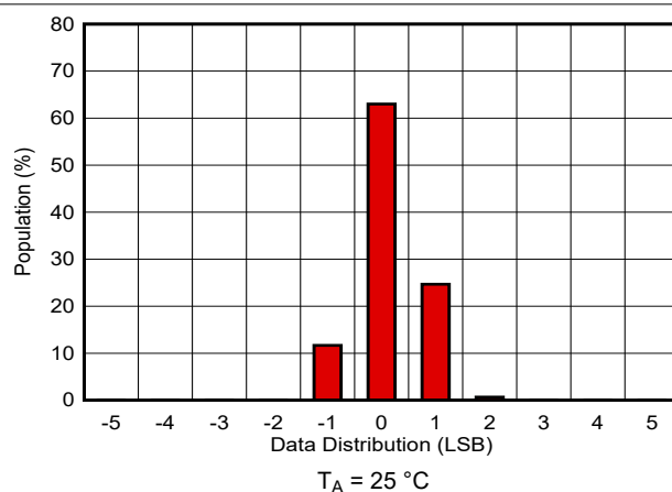
Figure 7-15. Data Distribution With 3.5-ms Conversion Time and Averaging On
