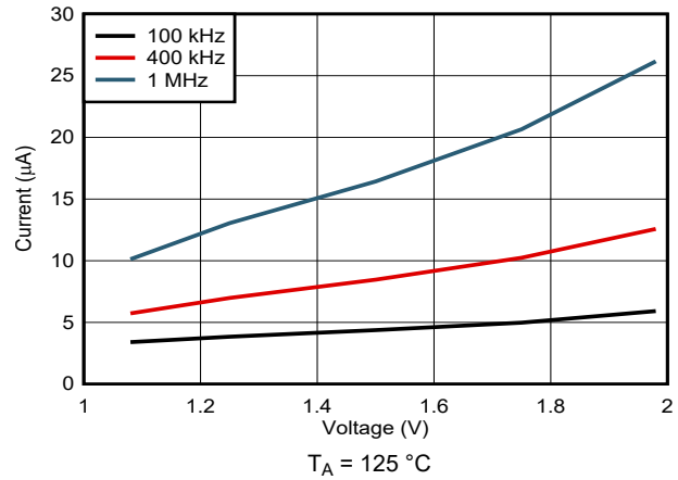
Figure 7-9. Supply Current vs. V_{DD} With Toggling SCL
