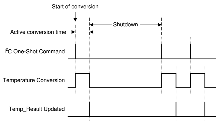
Figure 8-5. One-Shot Timing Diagram
