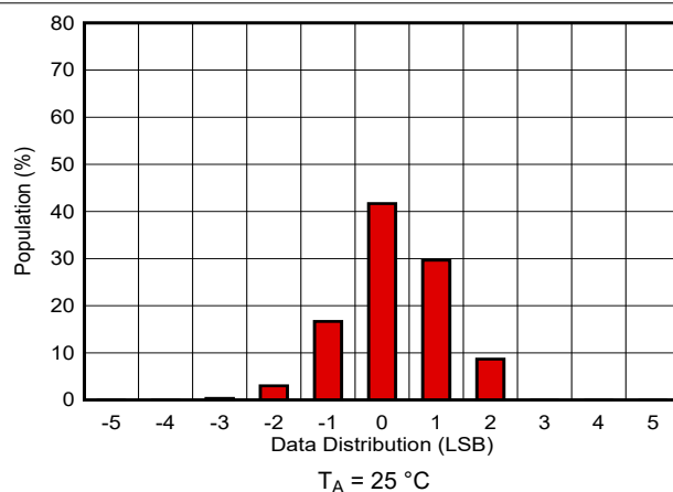
Figure 7-19. Data Distribution With 1.2-ms Conversion Time and Averaging On
