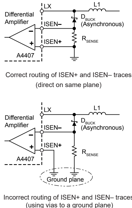
Figure 17. Comparison of routing paths for the traces between the A4407 ISEN+ and ISEN- traces and the sense resistor, R_{SENSE}
