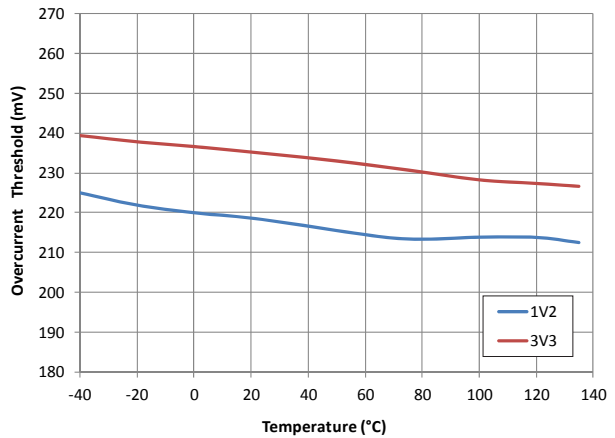
1V2 and 3V3 Overcurrent Threshold versus Temperature
