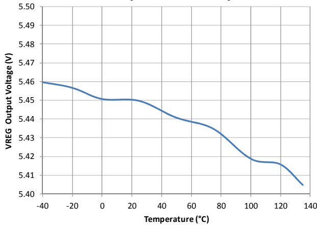
V5 Output versus Temperature
