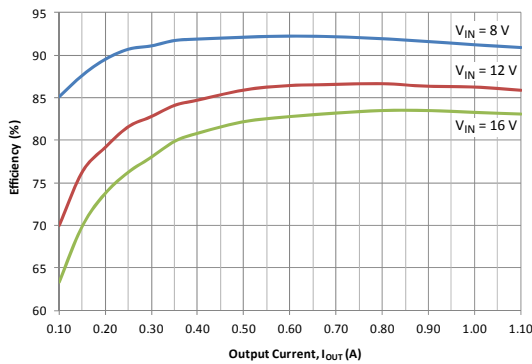
Buck Regulator (VREG) Efficiency
