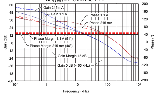
Buck Regulator Bode Plots
