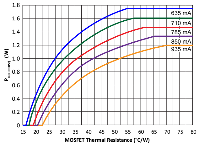
Figure 13. R_{DROP1} power dissipation versus 3.3 V MOSFET thermal resistance at various 3.3 V regulator maximum current settings
