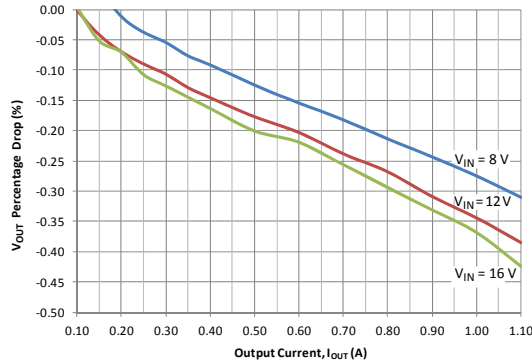
Buck Regulator (VREG) Load Regulation
