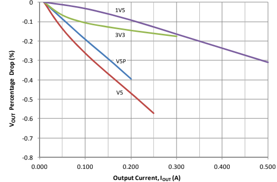
Linear Regulator Load Regulation
