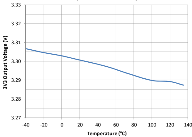
3V3 Output versus Temperature
