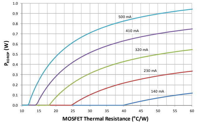
Figure 10. R_{\text{DROP}} Dissipation versus MOSFET thermal resistance at various V33 regulator maximum current settings, I_{\text{V33ILIM}}
