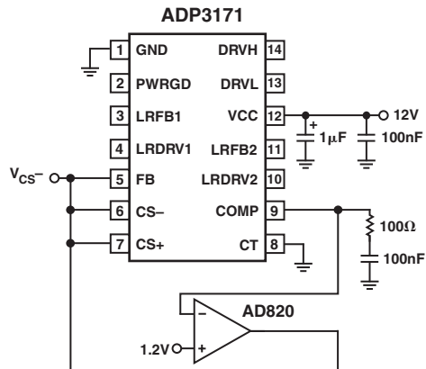
Figure 1. Closed-Loop Output Voltage Accuracy Test Circuit
