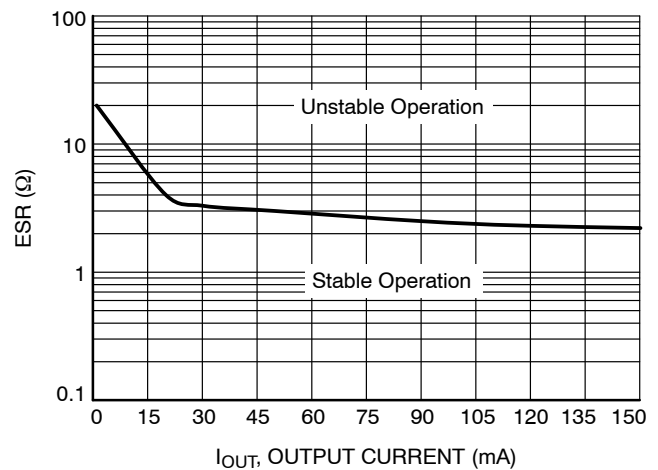
Figure 20. Maximum C_{OUT} ESR Value vs. Load Current
