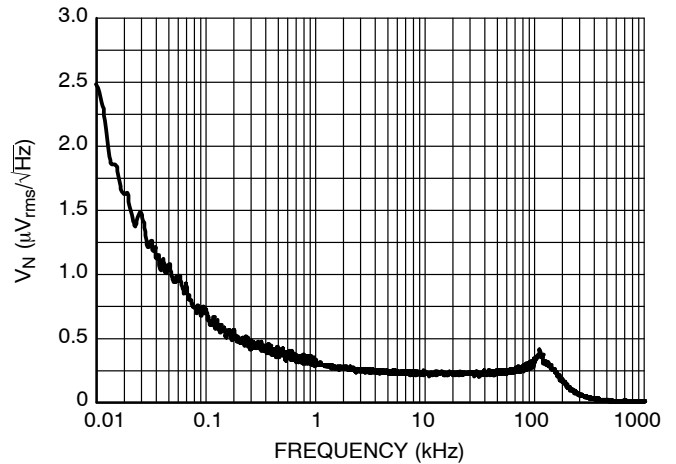
Figure 19. Output Voltage Noise, 1.5 V Version, V_{IN} = 2.6 V, I_{OUT} = 30 mA
