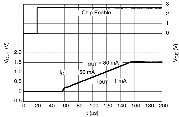
Figure 34. Start-up, 1.5 V Version, V_{IN} = 2.6 \text{ V}
