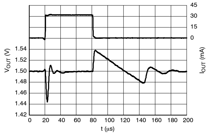
Figure 28. Load Transients, 1.5 V Version, I_{OUT} = 1 - 30 mA, t_R = t_F = 0.5 \mu s, V_{IN} = 2.6 V
