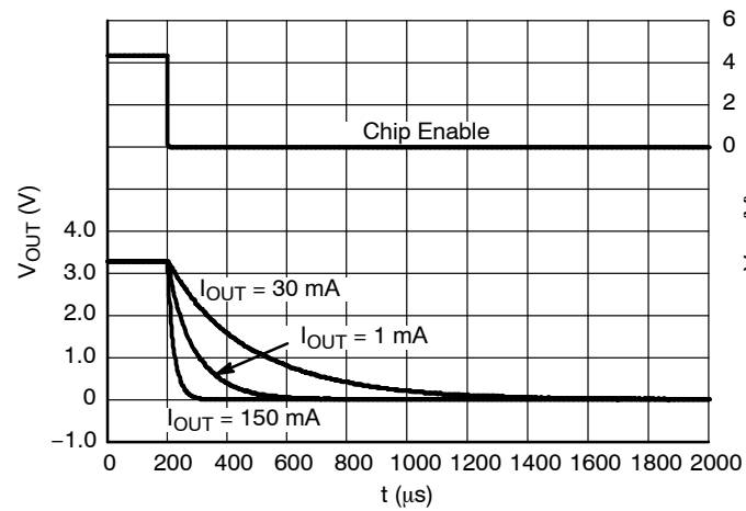
Figure 37. Shutdown, 3.3 V Version D, V_{IN} = 4.3 V
