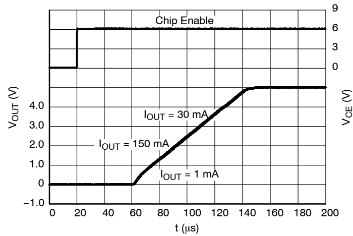
Figure 36. Start-up, 5.0 V Version, V_{IN} = 6.0 V
