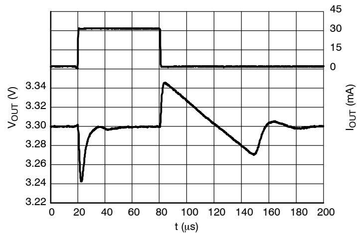
Figure 29. Load Transients, 3.3 V Version, I_{OUT} = 1 - 30 mA, t_R = t_F = 0.5 \mu s, V_{IN} = 4.3 V
