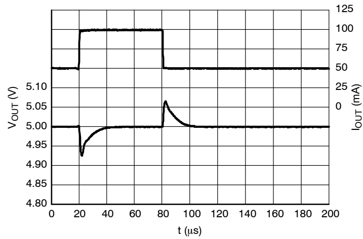
Figure 27. Load Transients, 5.0 V Version, I_{OUT} = 50 - 100 mA, t_R = t_F = 0.5 \mu s, V_{IN} = 6.0 V
