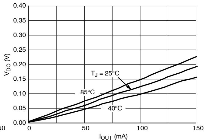
Figure 7. Dropout Voltage vs. Output Current 5.0 V Version
