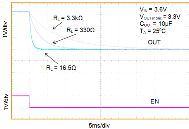
Figure 43. Enable Turn-Off Response, V_{OUT} = 3.3V , C_{OUT} = 10\mu F
