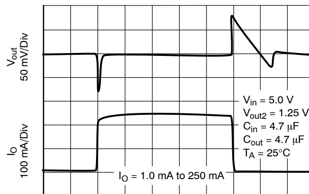
Figure 18. Load Transient Response for V_{out2}
