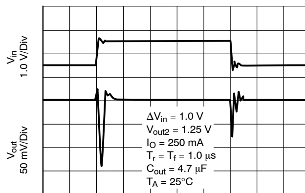
Figure 20. Line Transient Response for V_{out2}
