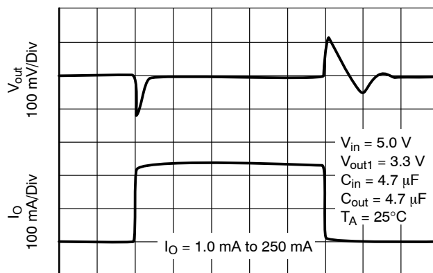
Figure 16. Load Transient Response for V_{out1}
