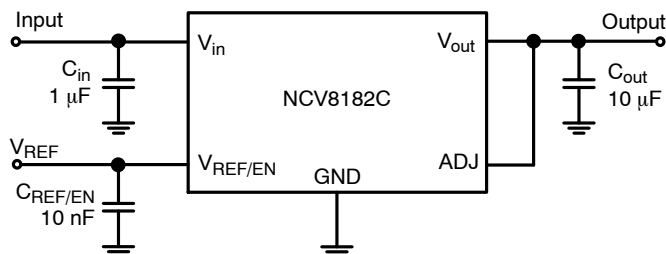
Figure 1. Application Circuit
