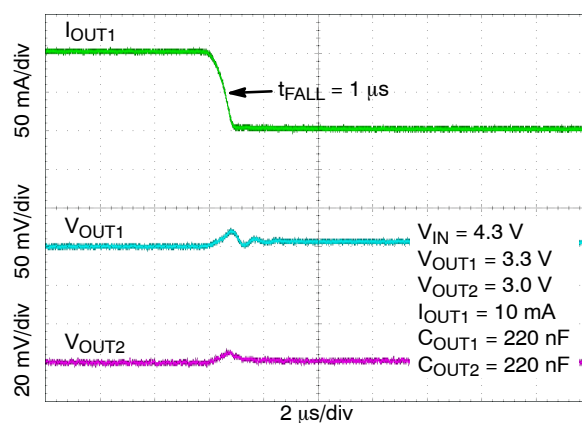
Figure 51. Load Transient Response – Falling Edge, I_{OUT} = 150 mA to 50 mA
