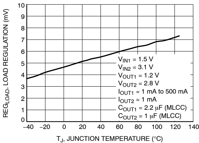
Figure 7. Load Regulation vs. Temperature – V OUT1 = 1.2 V
