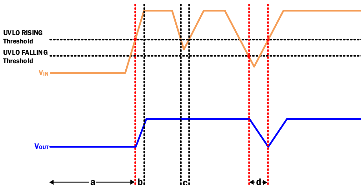
Figure 122. UVLO Operation
