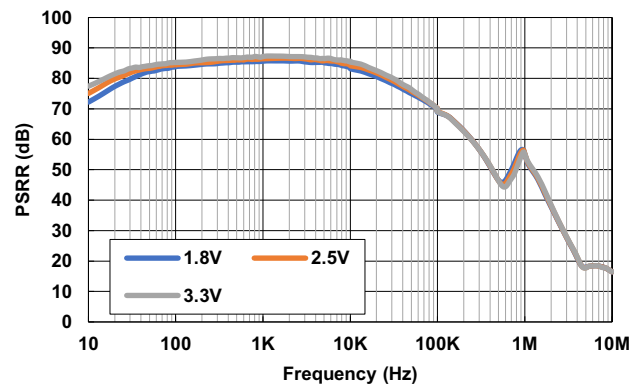
Figure 16. PSSR vs Frequency for Various V_{OUT} ( V_{IN} = V_{OUT} + 1.2V , I_{OUT} = 500mA )
