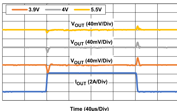
Figure 66. Load Transient Response for Various V_{IN} ( V_{OUT} = 3.3V , \Delta I_{OUT} = 100mA to 2A at 1A/\mu s )
