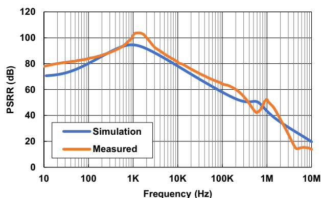
Figure 127. PSRR vs Frequency for SPICE Compared to Measured Results ( V_{IN} = 5V , V_{OUT} = 3.3V , I_{OUT} = 2A , C_{SET} = 1\mu F , C_{OUT} = 22\mu F )
