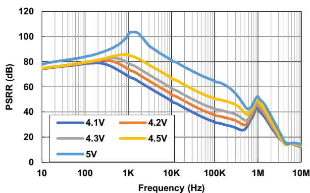
Figure 55. PSRR vs Frequency for Various V_{IN} ( V_{OUT} = 3.3V , I_{OUT} = 2A )
