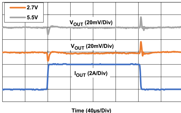
Figure 62. Load Transient Response for Various V_{IN} ( V_{OUT} = 1.8V , \Delta I_{OUT} = 100mA to 2A at 1A/\mu s )
