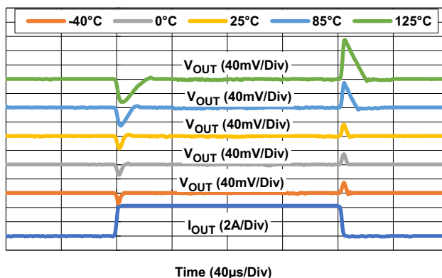
Figure 64. Load Transient Response for Various Temperatures ( V_{IN} = 3.8V , V_{OUT} = 3.3V , \Delta I_{OUT} = 100mA to 2A at 1A/\mu s )
