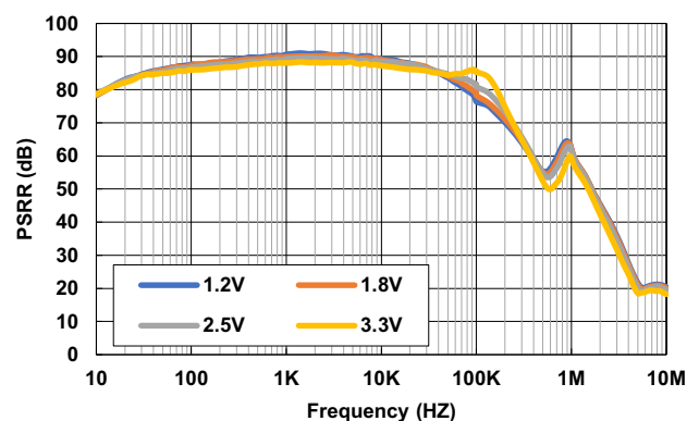
Figure 18. PSSR vs Frequency for Various V_{OUT} ( V_{IN} = 5V , I_{OUT} = 500mA )
