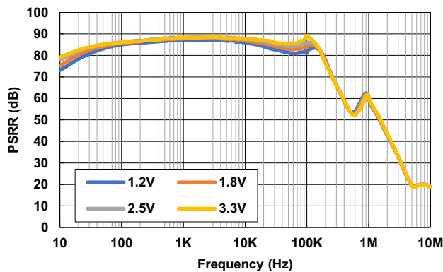
Figure 15. PSSR vs Frequency for Various V_{OUT} ( V_{IN} = V_{OUT} + 2V , I_{OUT} = 500mA )
