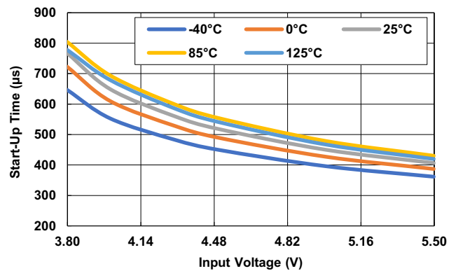
Figure 111. Start-Up Time vs Input Voltage ( V_{OUT} = 3.3V , C_{SET} = 1\mu F , C_{OUT} = 22\mu F , I_{OUT} = 2A )
