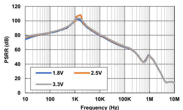
Figure 20. PSSR vs Frequency for Various V_{OUT} ( V_{IN} = V_{OUT} + 1.7V , I_{OUT} = 2A )
