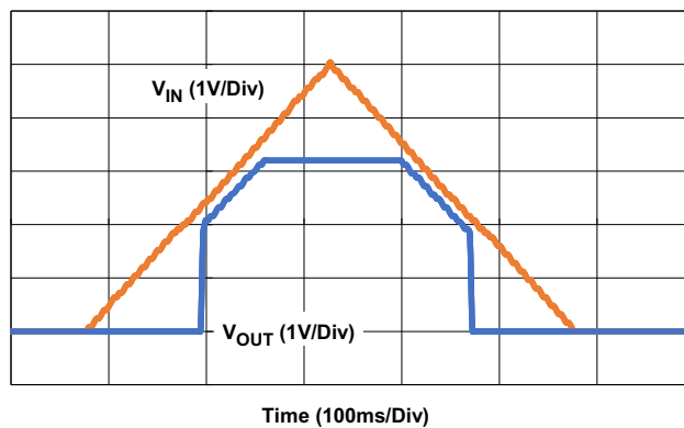
Figure 120. Input Supply Slow Ramp Up and Ramp Down (\Delta V_{IN} = 0V \text{ to } 5V, V_{OUT} = 3.3V, I_{OUT} = 2A, C_{SET} = 1\mu F, C_{OUT} = 22\mu F)
