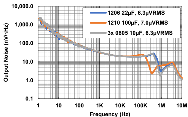
Figure 14. Output Noise vs Frequency for Various C_{OUT} ( V_{IN} = V_{OUT} + 1V , I_{OUT} = 2A )
