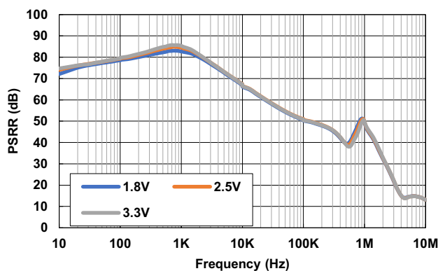
Figure 19. PSSR vs Frequency for Various V_{OUT} ( V_{IN} = V_{OUT} + 1.2V , I_{OUT} = 2A )
