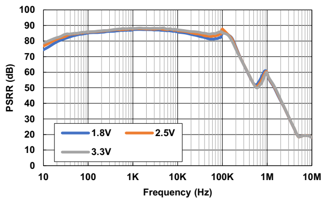
Figure 17. PSSR vs Frequency for Various V_{OUT} ( V_{IN} = V_{OUT} + 1.7V , I_{OUT} = 500mA )
