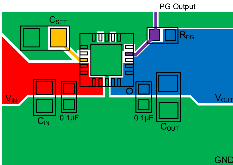
Figure 126. Layout Scheme
