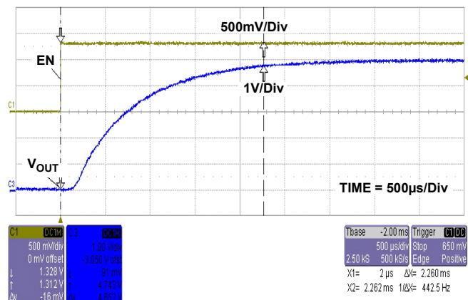
Figure 9. Start-Up Waveform
