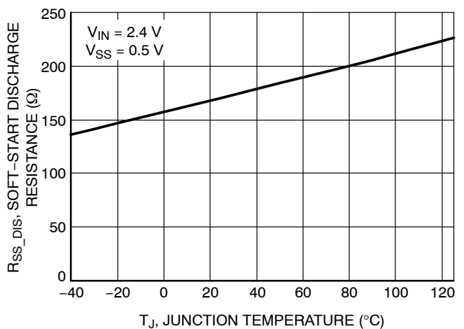
Figure 21. Soft-Start Discharging Resistance vs. Temperature
