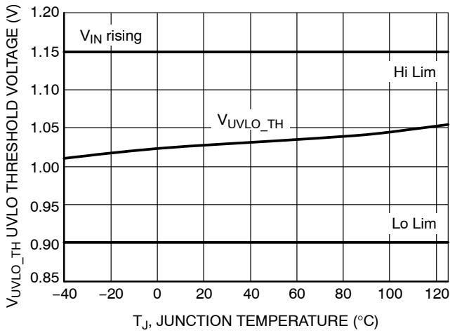
Figure 22. UVLO Threshold Voltage vs. Temperature
