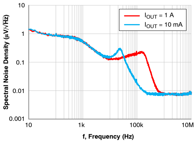
Figure 11. Output Voltage Spectral Noise Density vs. Frequency – V_{OUT(NOM)} = 1.0\text{ V}
