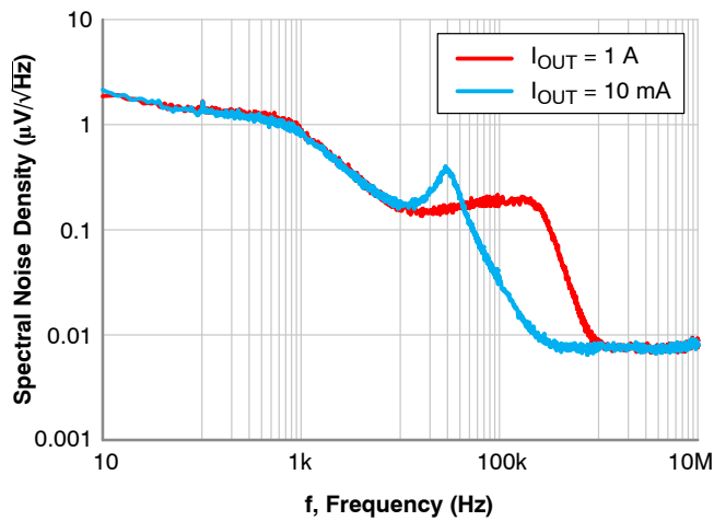
Figure 12. Output Voltage Spectral Noise Density vs. Frequency – V_{OUT(NOM)} = 1.8\text{ V}
