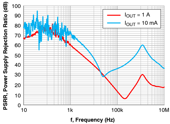
Figure 9. PSRR vs. Frequency – V_{OUT(NOM)} = 1.0\text{ V}
