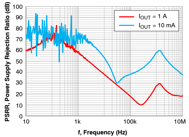
Figure 10. PSRR vs. Frequency – V_{OUT(NOM)} = 1.8\text{ V}
