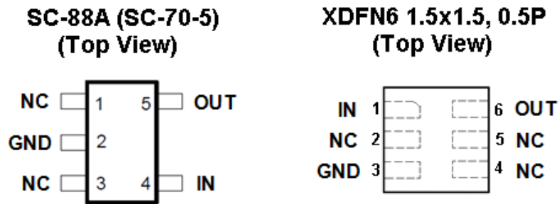
Figure 3. Pin Description
