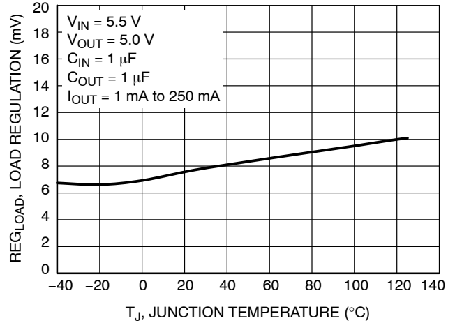
Figure 10. Load Regulation vs. Temperature – V_{OUT} = 5.0\text{ V}
