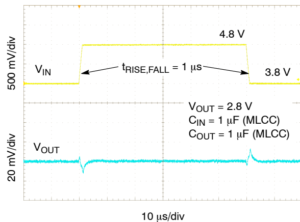
Figure 35. Line Transient Response – I_{OUT} = 300 \text{ mA}
