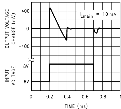
Line Transient Response (Main Regulator)
