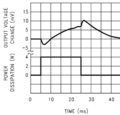
Thermal Regulation (Main Regulator)
