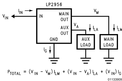
FIGURE 1. Current/Voltage Diagram
