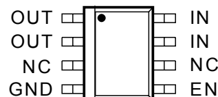
MIC5200-x.xBM (SOIC-8)
