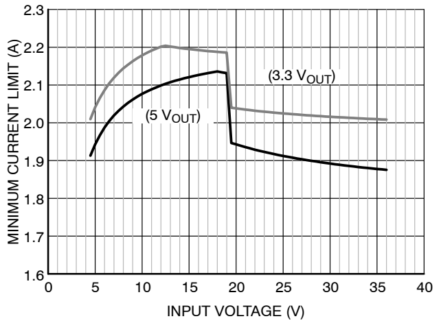
Figure 26. NCV890230 Load Current Capability with 4.7 \mu H Inductor
