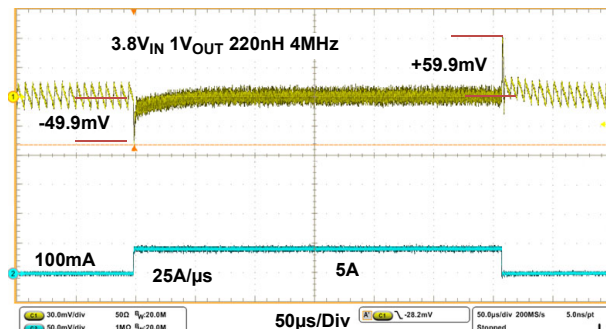
V_{IN} = 3.8V , V_{OUT} = 1V Load Step Slew Rate: 25A/μs, 0.1A to 5A 220nH Inductor (Cyntec) 1x22μF Capacitor (0603 6.3V Murata) 6x4.3μF Capacitor (Low ESL)
