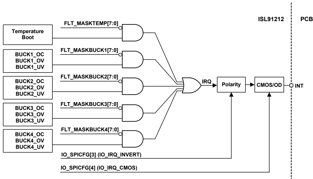
Figure 39. Interrupt Tree
