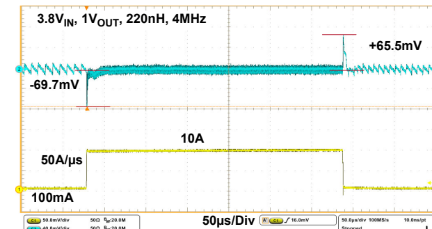
V_{IN} = 3.8V , V_{OUT} = 1V Load Step Slew Rate: 50A/μs, 0.1A to 10A 220nH Inductor (Cyntec) 3x22μF Capacitor (0603 6.3V Murata) 6x4.7μF Capacitor (0603 10V)
