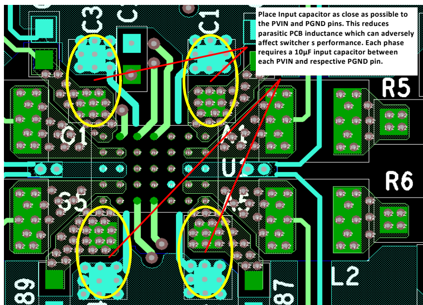
Figure 45. Recommended PCB Layout Top Layer
