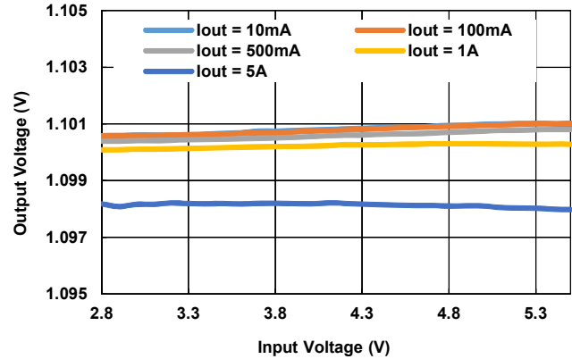
Figure 13. Single-Phase V_{OUT} vs V_{IN} (10mA to 5A)
