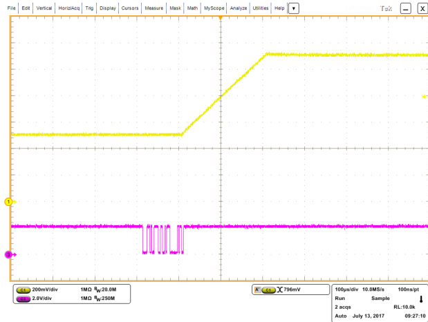
Figure 17. 0.5V to 1.1V DVS; Load = 5A, Slew Rate = 3mV/μs
