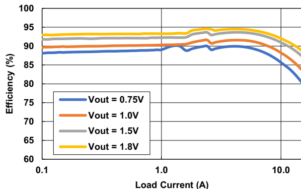
Figure 8. 3-Phase Configuration Efficiency ( V_{IN} = 3.3V , f_{SW} = 2MHz )
