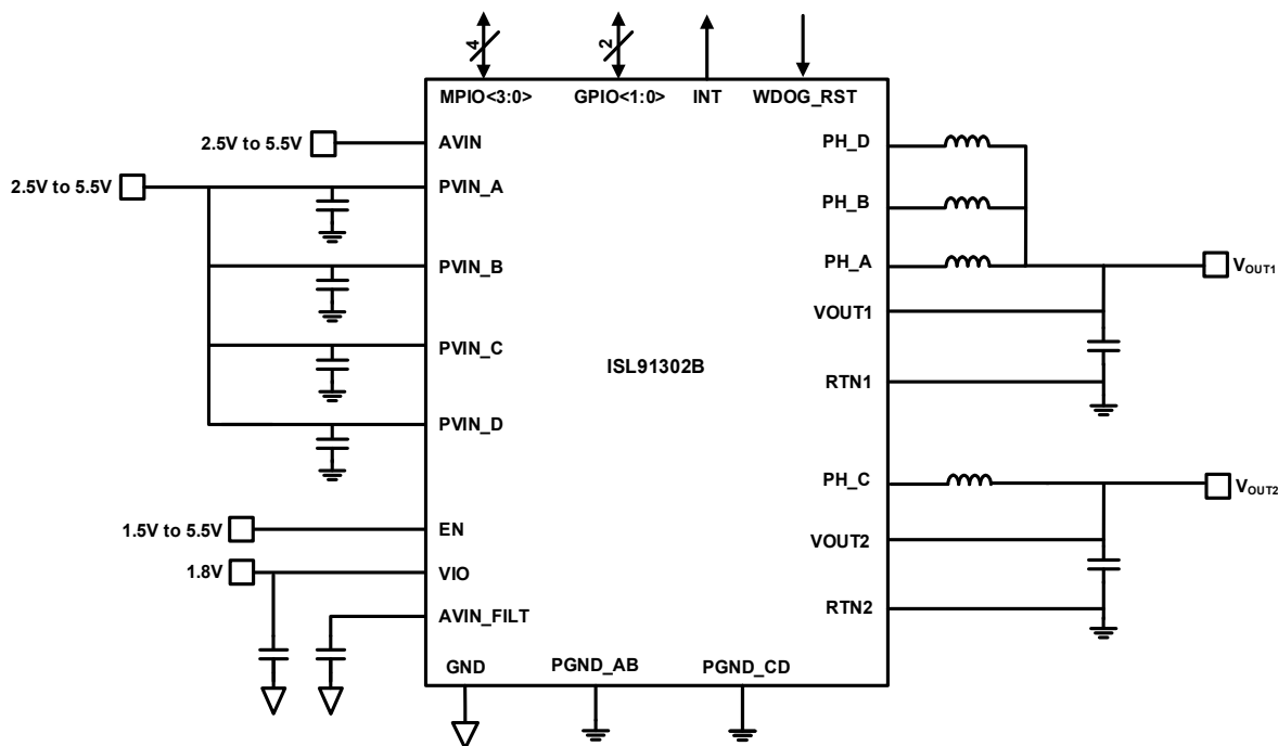
Figure 3. Typical Application Circuit: 3-Phase + 1-Phase
