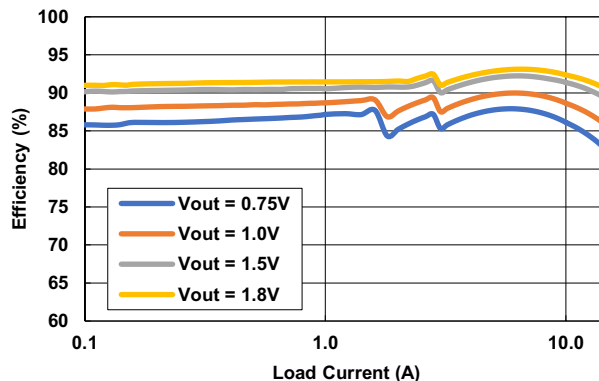
Figure 9. 3-Phase Configuration Efficiency ( V_{IN} = 5.0V , f_{SW} = 2MHz )
