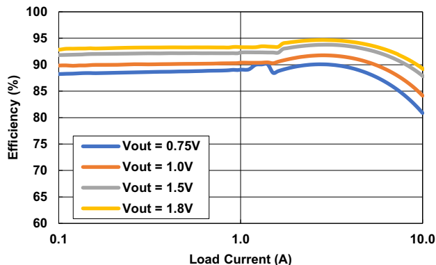
Figure 6. 2-Phase Configuration Efficiency ( V_{IN} = 3.3V , f_{SW} = 2MHz )
