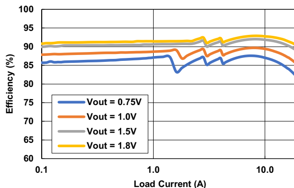
Figure 11. 4-Phase Configuration Efficiency ( V_{IN} = 5.0V , f_{SW} = 2MHz )
