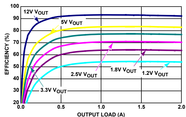
FIGURE 5. EFFICIENCY vs LOAD (24V INPUT - 500kHz)
