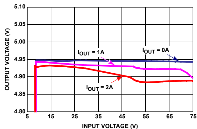
FIGURE 17. OUTPUT VOLTAGE REGULATION vs V_{IN} ( V_{OUT} = 5V - 500kHz )
