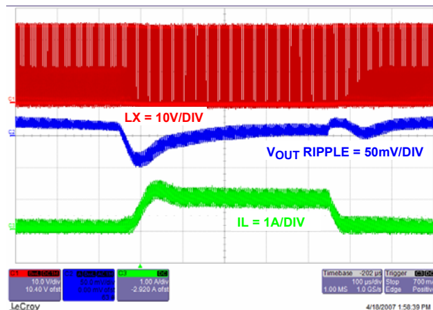
FIGURE 23. LOAD TRANSIENT
