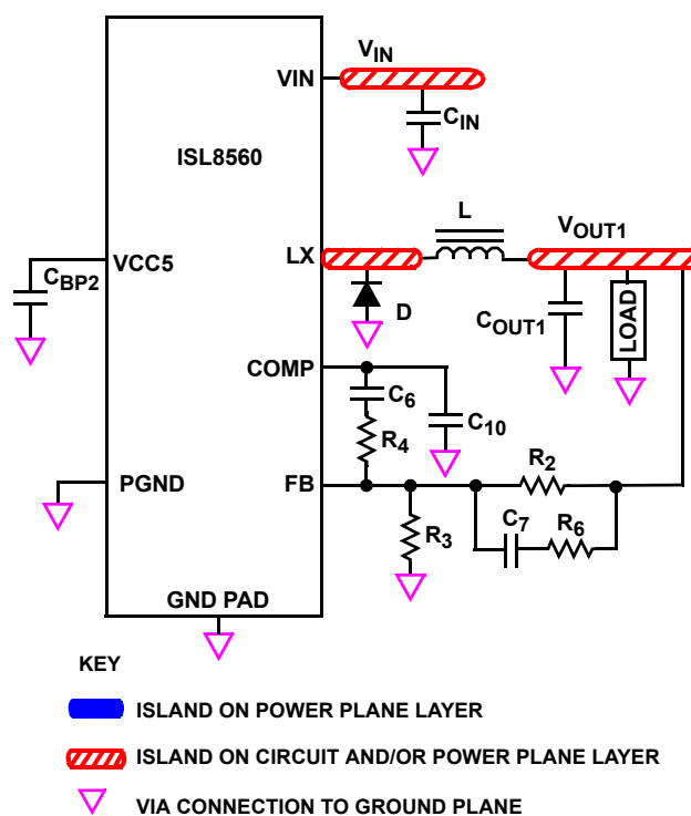
FIGURE 32. PRINTED CIRCUIT BOARD POWER PLANES AND ISLANDS
