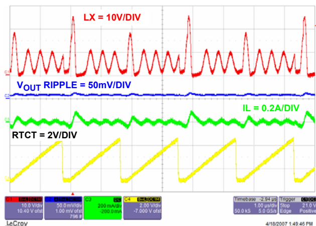
FIGURE 21. STEADY STATE OPERATION AT NO LOAD
