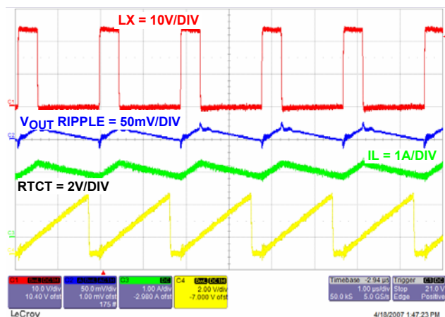
FIGURE 22. STEADY STATE OPERATION WITH FULL LOAD
