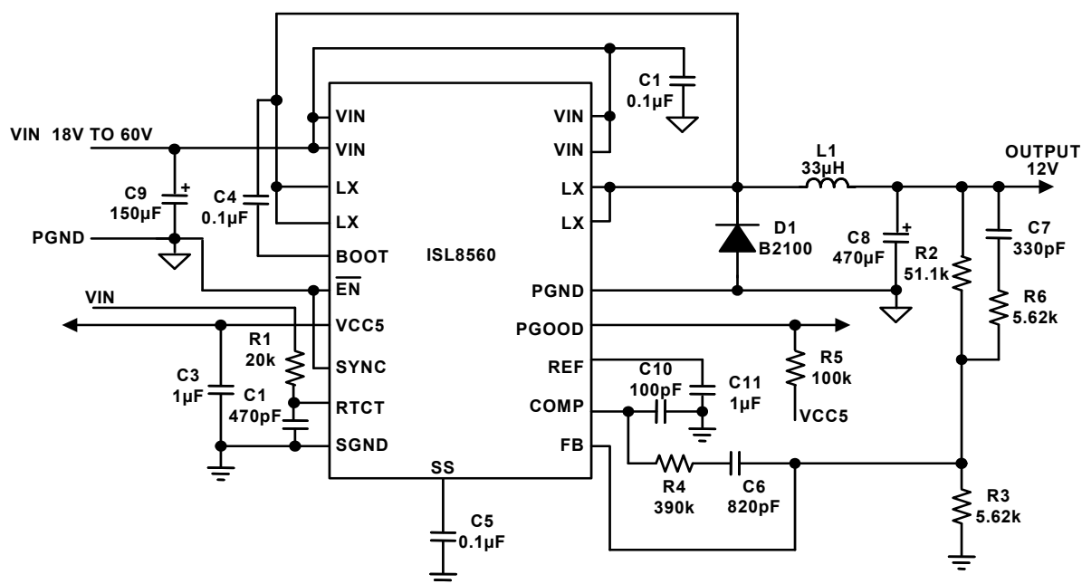
FIGURE 3. TYPICAL SCHEMATIC FOR ISL8560 (12V V OUT )
