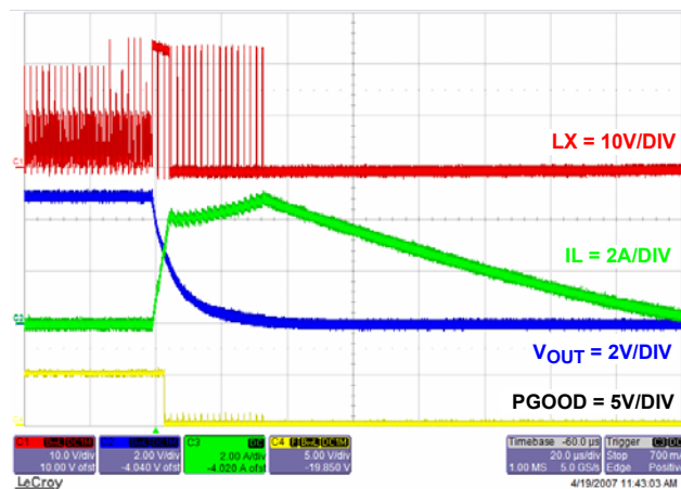
FIGURE 27. OUTPUT SHORT CIRCUIT
