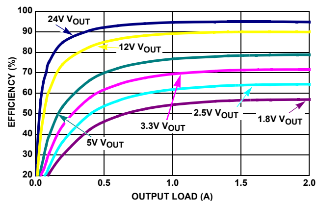
FIGURE 7. EFFICIENCY vs LOAD (48V INPUT - 500kHz)
