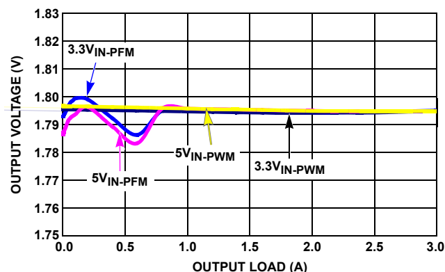
FIGURE 12. V_{\text{OUT}} REGULATION vs LOAD (1MHz, V_{\text{OUT}} = 1.8\text{V} )
