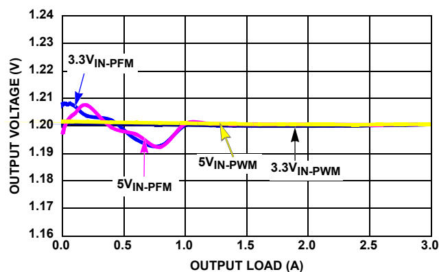
FIGURE 10. V_{\text{OUT}} REGULATION vs LOAD (1MHz, V_{\text{OUT}} = 1.2\text{V} )
