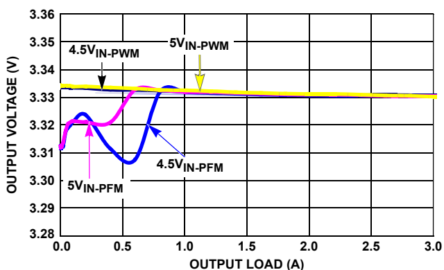
FIGURE 14. V_{\text{OUT}} REGULATION vs LOAD (1MHz, V_{\text{OUT}} = 3.3\text{V} )
