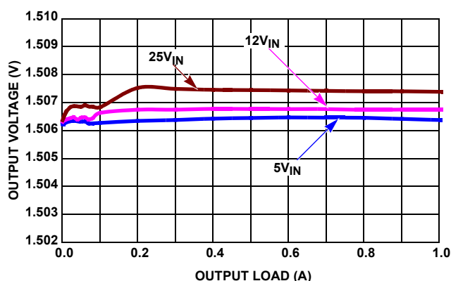
FIGURE 8. V OUT REGULATION vs LOAD, 500kHz, 1.5V OUT
