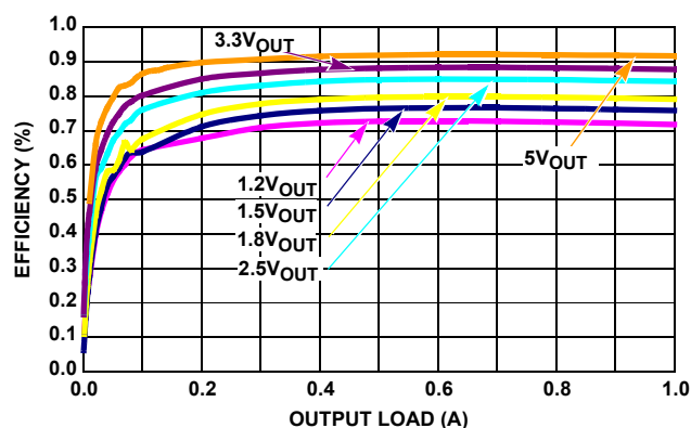
FIGURE 4. EFFICIENCY vs LOAD, 500kHz, 12V IN
