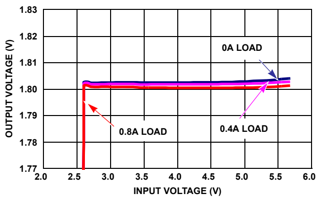
FIGURE 13. OUTPUT VOLTAGE REGULATION vs V_{IN} 1.8V_{OUT} PWM MODE
