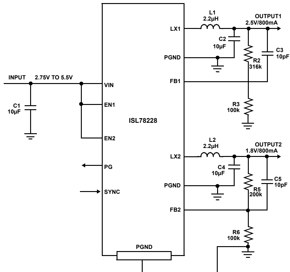
FIGURE 2. TYPICAL APPLICATION
