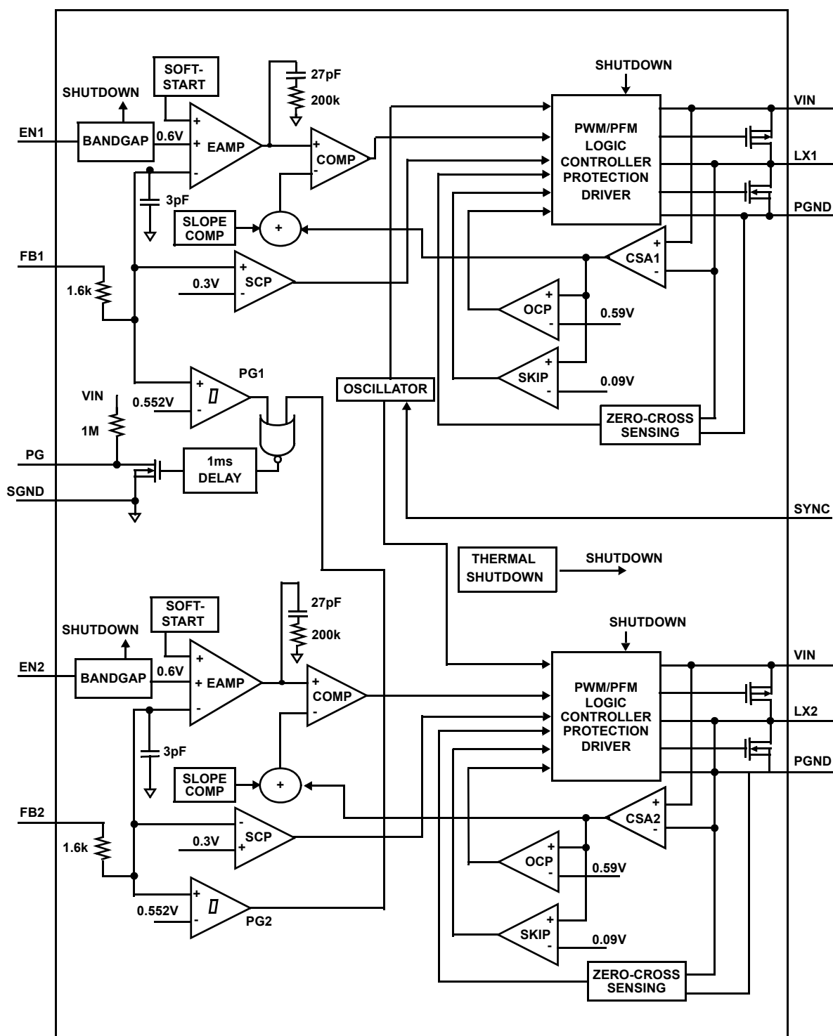
FIGURE 44. BLOCK DIAGRAM
