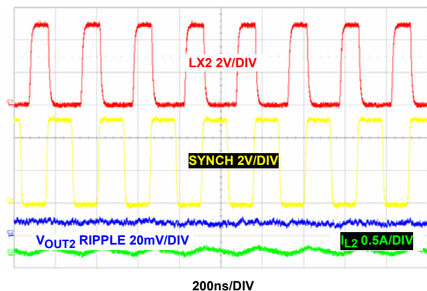
FIGURE 35. CH2 STEADY STATE OPERATION AT NO LOAD (PFM) WITH FREQUENCY = 4MHz
