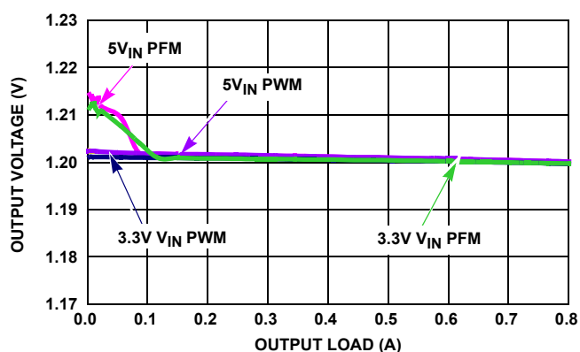
FIGURE 8. V_{OUT} REGULATION vs LOAD 2.25MHz, 1.2VOUT PFM
