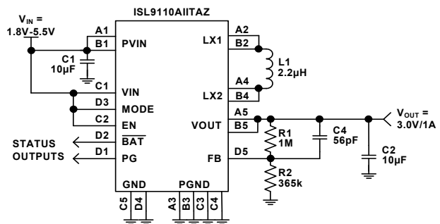
FIGURE 31. TYPICAL ISL9110AIITAZ APPLICATION
