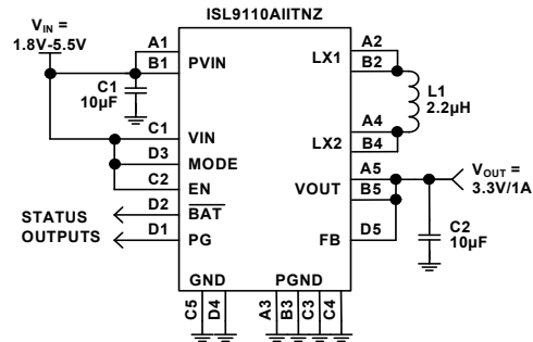
FIGURE 30. TYPICAL ISL9110AIITNZ APPLICATION
