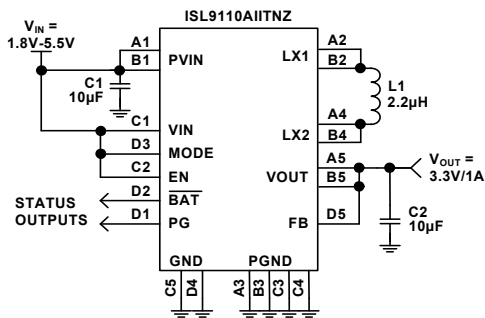
FIGURE 29. TYPICAL ISL9110AIITNZ APPLICATION
