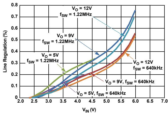
Figure 11. Line Regulation
