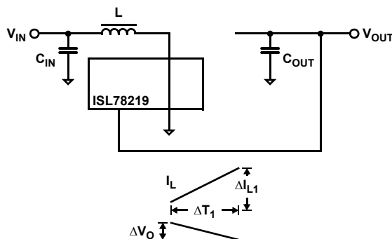
Figure 15. Boost Converter - Cycle 1, Power Switch Closed
