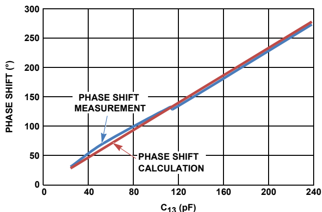
FIGURE 36. PHASE SHIFT vs CAPACITANCE
