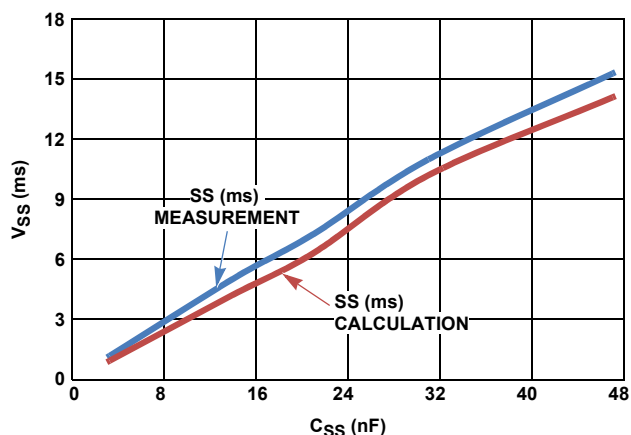
FIGURE 37. SOFT-START TIME vs C_{SS}
