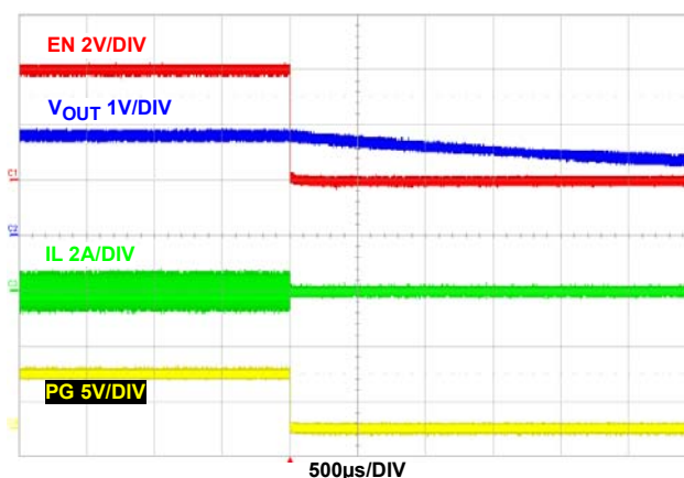
FIGURE 25. SOFT-DISCHARGE SHUTDOWN
