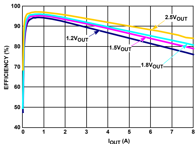
FIGURE 4. EFFICIENCY vs LOAD (1MHz 3.3VIN PWM)
