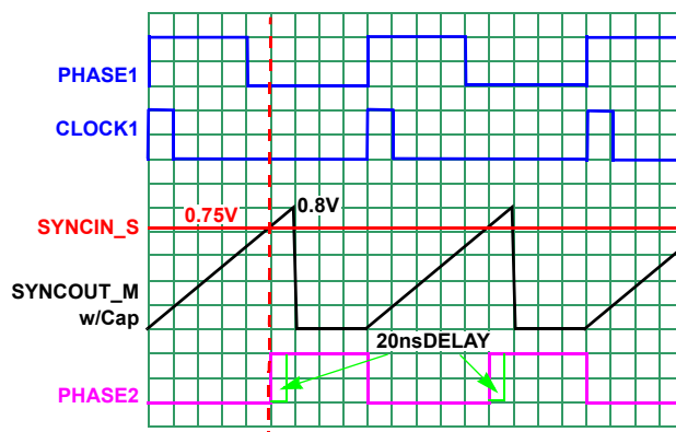
FIGURE 35. SYNCHRONIZATION WAVEFORMS
