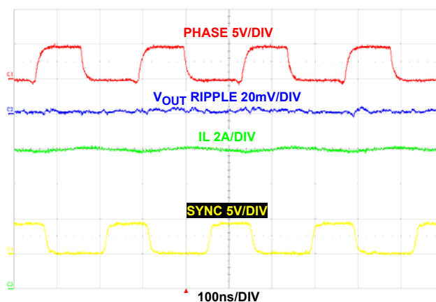
FIGURE 29. STEADY STATE OPERATION AT FULL LOAD (PWM) WITH FREQUENCY = 4MHz
