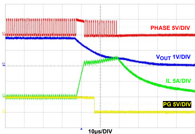
FIGURE 30. OUTPUT SHORT-CIRCUIT
