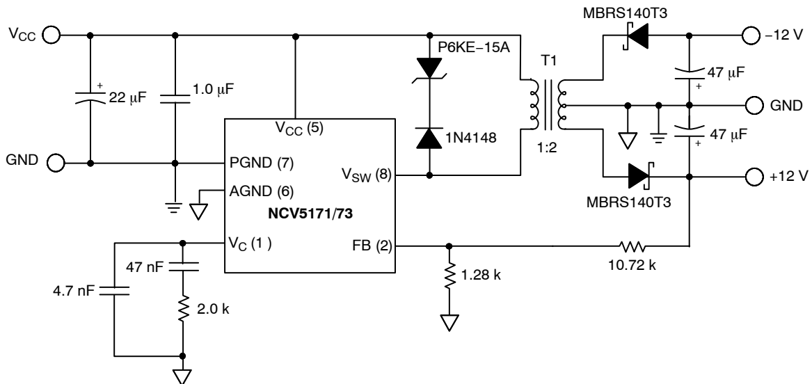
Figure 36. Additional Application Diagram, 2.7 to 13 V Input, \pm 12 V/ 200 mA Output Flyback Converter
