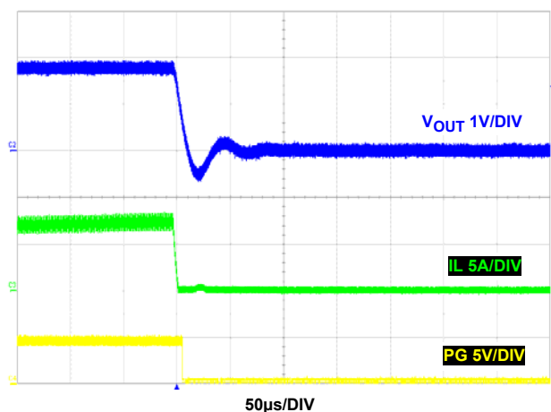
FIGURE 43. OVERCURRENT PROTECTION
