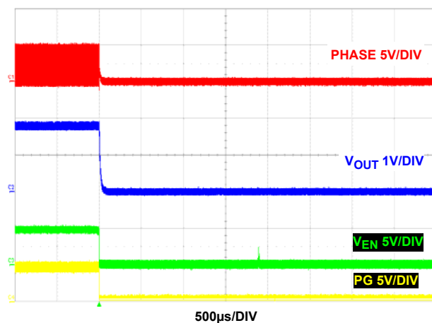
FIGURE 24. SHUTDOWN AT 5A LOAD (PWM)
