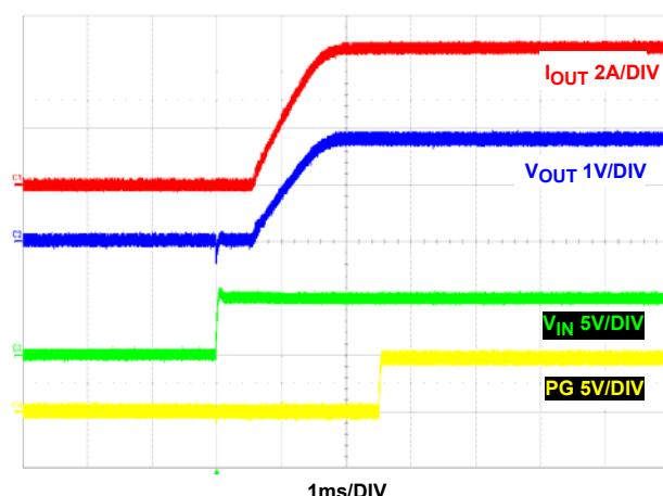
FIGURE 28. START-UP V_{IN} AT 5A LOAD (PWM)
