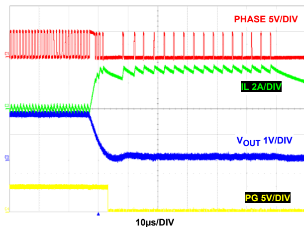
FIGURE 42. OUTPUT SHORT CIRCUIT
