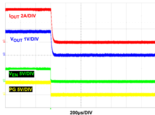
FIGURE 26. SHUTDOWN AT 5A LOAD (PFM)
