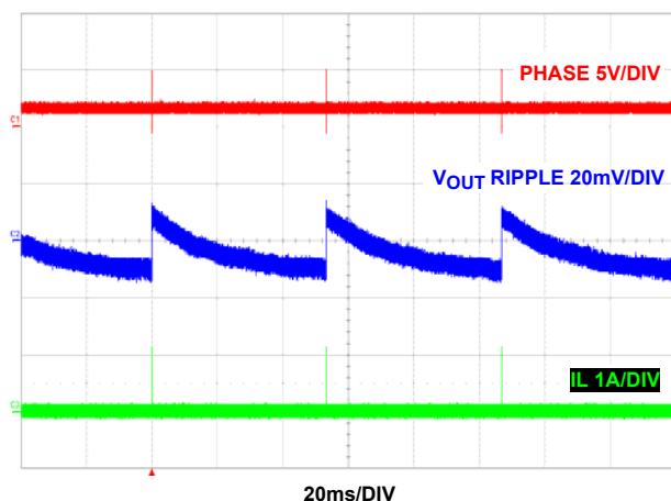
FIGURE 38. STEADY STATE AT NO LOAD PFM
