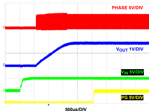
FIGURE 32. START-UP V_{\text{IN}} AT NO LOAD (PWM)
