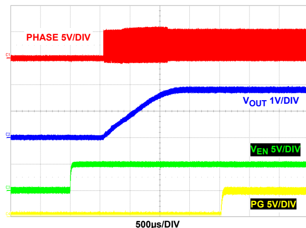
FIGURE 20. START-UP AT NO LOAD (PWM)
