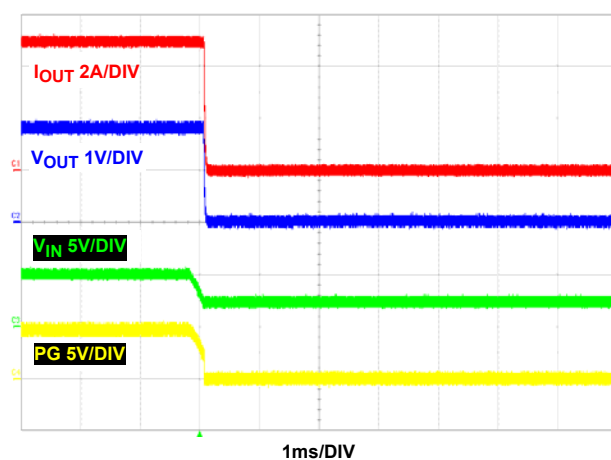
FIGURE 30. SHUTDOWN V_{IN} AT 5A LOAD (PWM)
