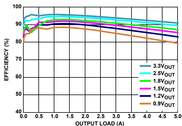
FIGURE 11. EFFICIENCY vs LOAD (2MHz 5VIN PFM)
