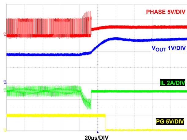
FIGURE 46. OVERVOLTAGE PROTECTION
