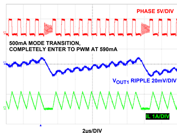
FIGURE 44. PFM TO PWM TRANSITION
