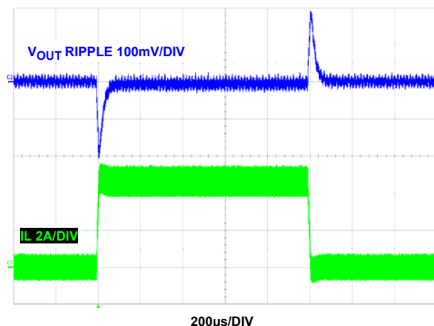
FIGURE 40. LOAD TRANSIENT (PWM)
