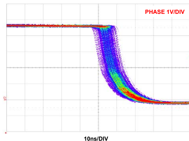
FIGURE 36. JITTER AT FULL LOAD PWM
