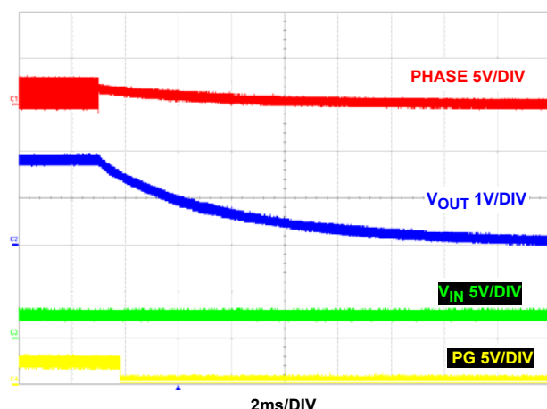
FIGURE 34. SHUTDOWN V_{\text{IN}} AT NO LOAD (PWM)
