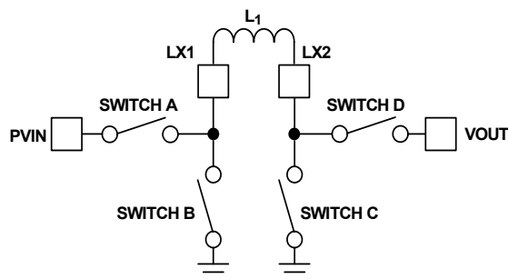
FIGURE 18. BUCK-BOOST TOPOLOGY
