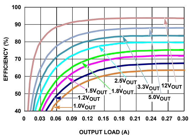
FIGURE 8. EFFICIENCY vs LOAD, PWM, V_{IN} = 24\text{V}
