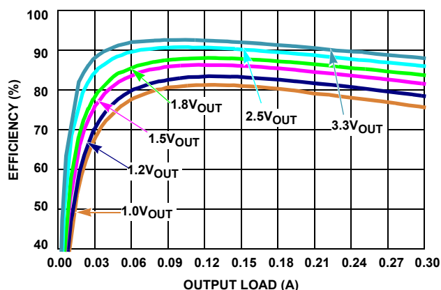
FIGURE 4. EFFICIENCY vs LOAD, PWM, V_{IN} = 5\text{V}
