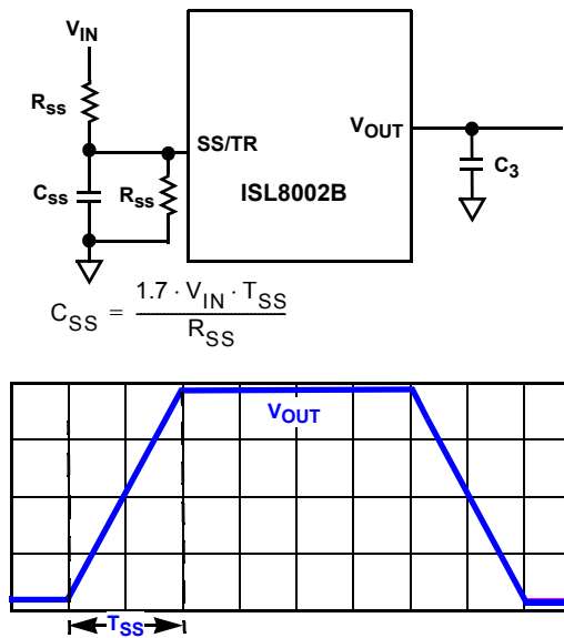
FIGURE 58. PROGRAMMING SOFT-START
