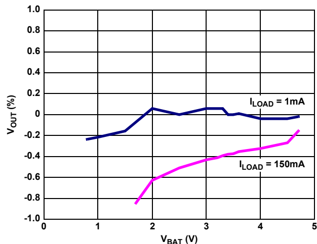
FIGURE 6. LINE REGULATION, V_{OUT} = 5V
