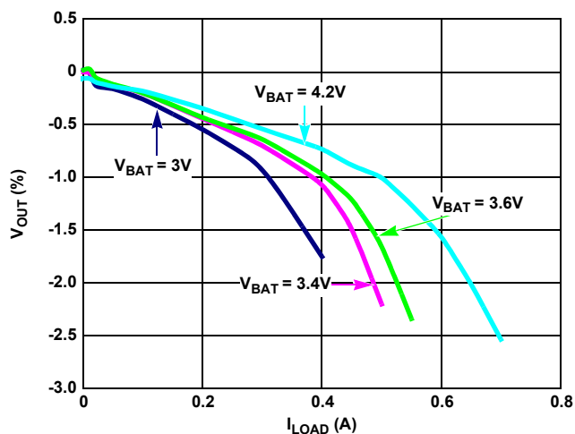
FIGURE 16. LOAD REGULATION
