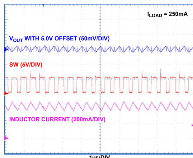
FIGURE 10. OUTPUT RIPPLE VOLTAGE ( I_{LOAD} = 250mA )
