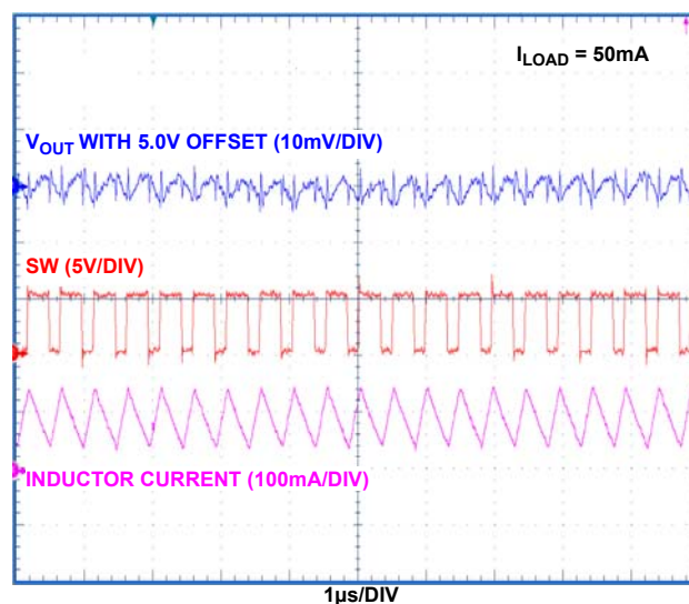
FIGURE 8. OUTPUT RIPPLE VOLTAGE ( I_{LOAD} = 50mA )
