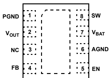
ISL78113A ADJUSTABLE OUTPUT (8 LD DFN) TOP VIEW
