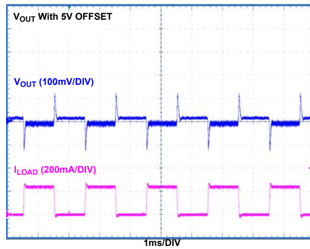
FIGURE 14. LOAD TRANSIENT RESPONSE (20mA TO 250mA)
