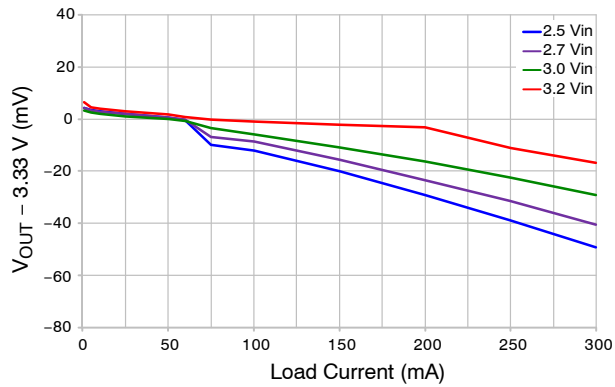
Figure 6. Line and Load Regulation
