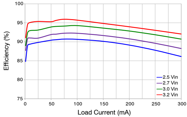
Figure 4. Efficiency vs. V_{IN}
