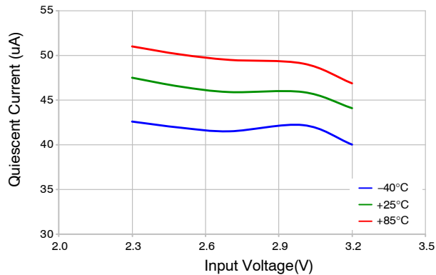
Figure 8. Quiescent Current
