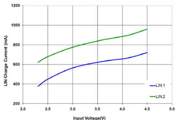
Figure 17. LIN Mode Current vs. V_{IN}
