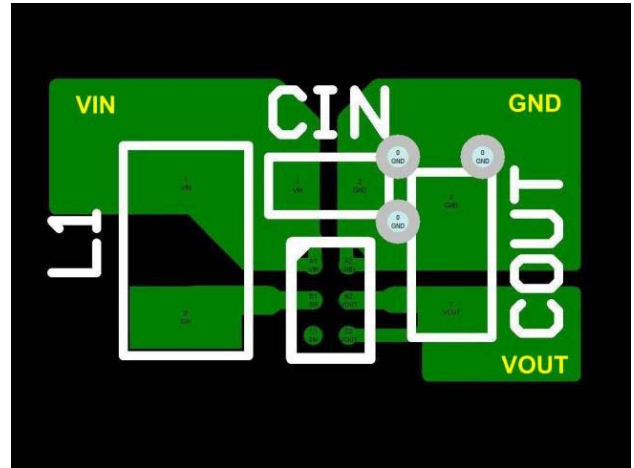
Figure 20. WLCSP Suggested Layout (Top View)
