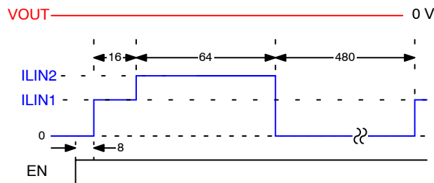
Figure 15. Fault Response into Short Circuit
