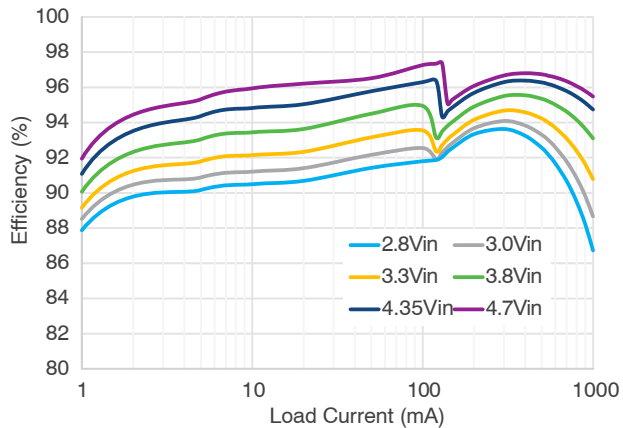
Figure 8. Efficiency vs. Load Current and Input Voltage, L = DFE201610R-H-1R0M
