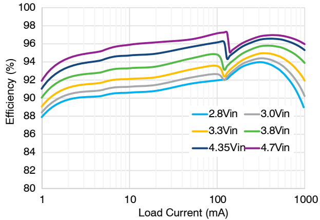
Figure 6. Efficiency vs. Load Current and Input Voltage, L = DFE201610E-1R0M
