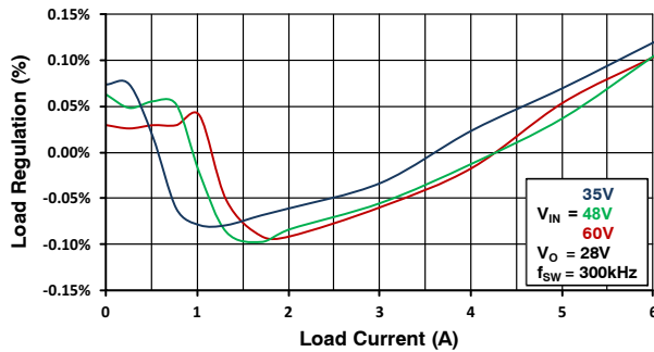
Figure 38. Load Regulation
