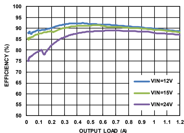
FIGURE 2. EFFICIENCY vs LOAD, PFM, V_{OUT} = 5V , L_1 = 22\mu\text{H}
