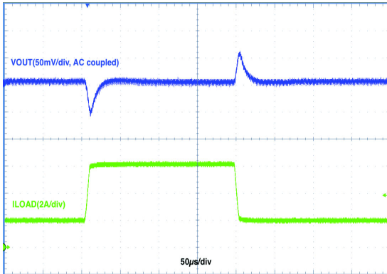
Figure 9. Load Transient, 2 A <-> 6 A, Slew Rate = 1 A/ \mu s
