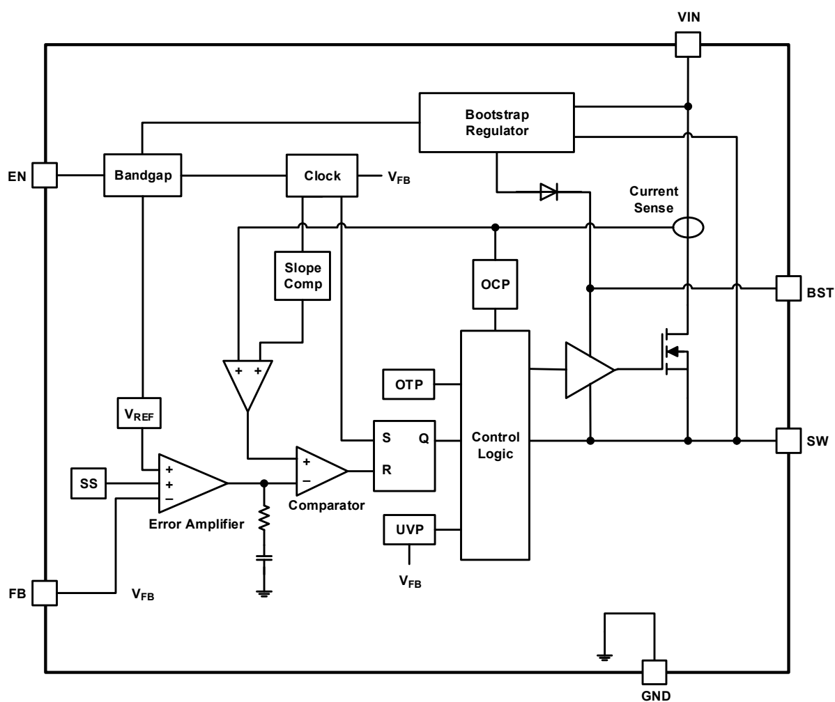
Figure 2. RAA211605 Block Diagram
