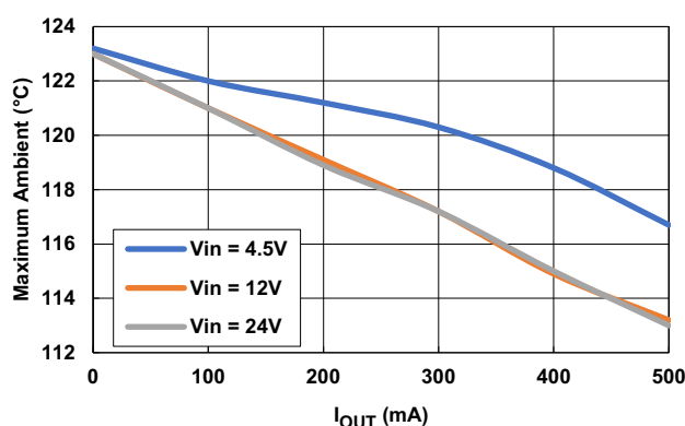
Figure 21. Maximum Ambient Temperature vs Output Current
