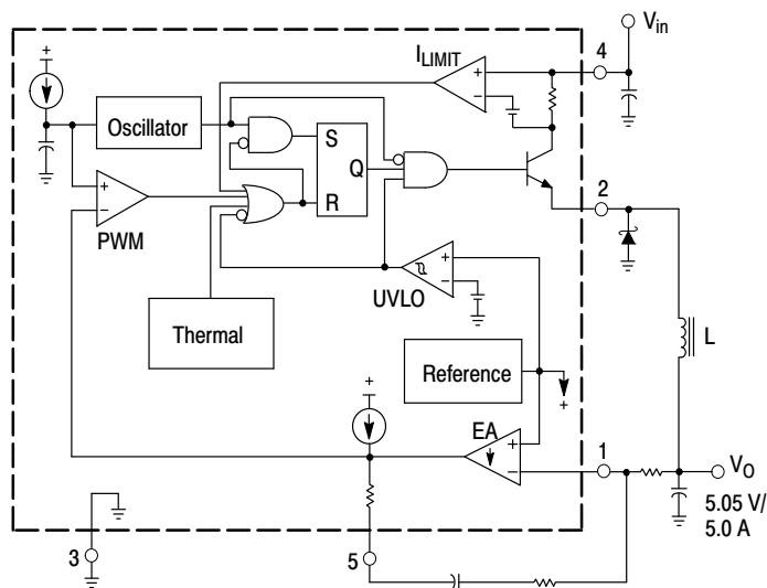
Figure 1. Simplified Block Diagram (Step Down Application)
