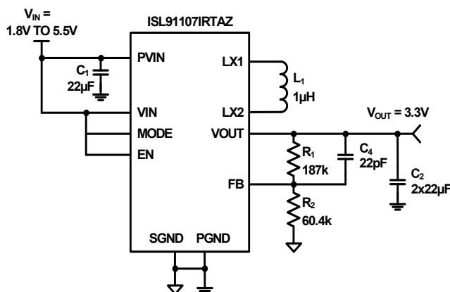
FIGURE 23. TYPICAL APPLICATION
