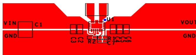
FIGURE 24. RECOMMENDED LAYOUT
