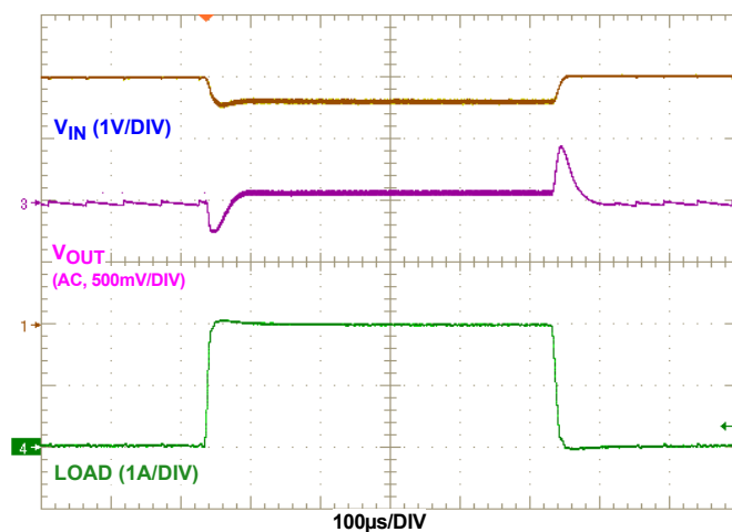
FIGURE 19. 0A TO 2A LOAD TRANSIENT, V_{IN} = 3.6\text{V} , V_{OUT} = 5\text{V}
