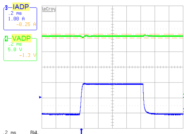
Figure 18. Reverse Mode, 20V ADP , 12V SYS , 0A-2A Transient Load
