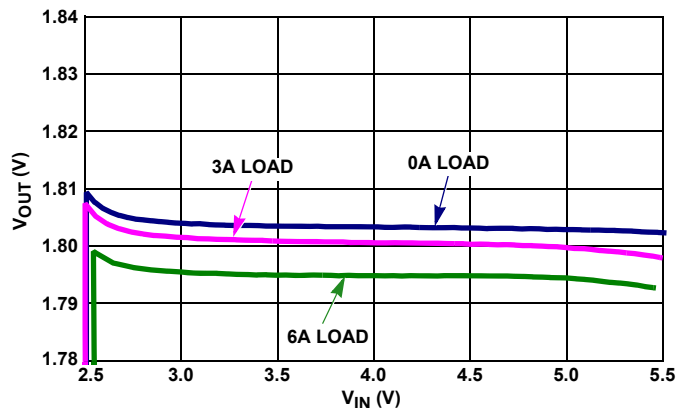
FIGURE 10. V_{OUT} REGULATION vs V_{IN} (PWM V_{OUT} = 1.8\text{V} )
