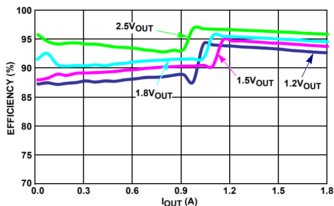
FIGURE 6. EFFICIENCY vs LOAD (1MHz 3.3VIN PFM)
