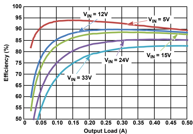
Figure 21. Efficiency vs Load, PWM, V_{OUT} = 3.3V
