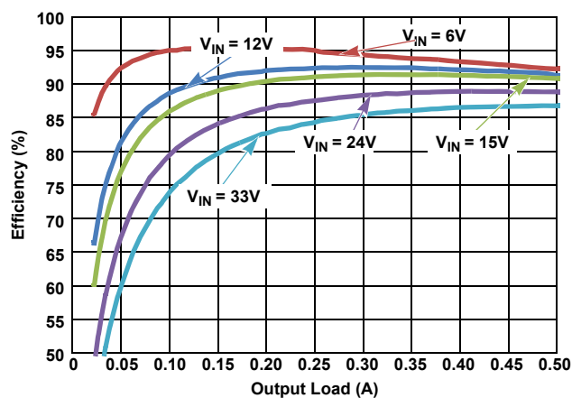
Figure 19. Efficiency vs Load, PMW, V_{OUT} = 5V
