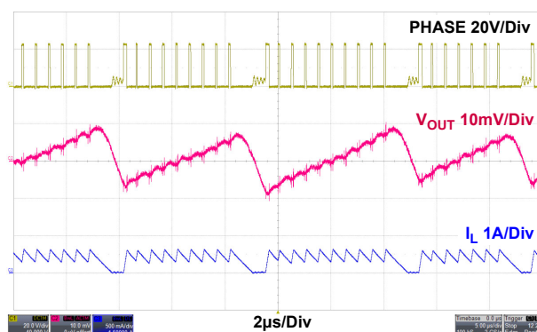
Figure 50. PFM to PWM Transition
