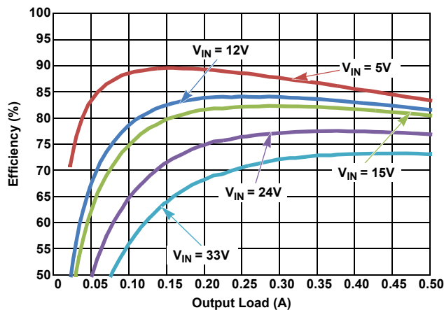
Figure 23. Efficiency vs Load, PWM, V_{OUT} = 1.8V
