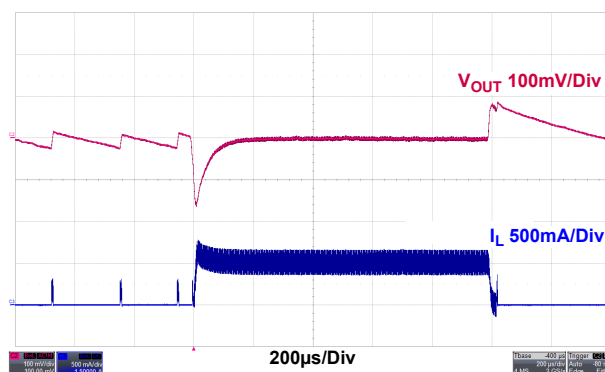
Figure 48. Load Transient, PFM
