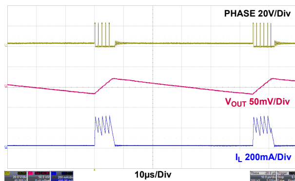
Figure 46. Light Load Operation at 20mA, PFM
