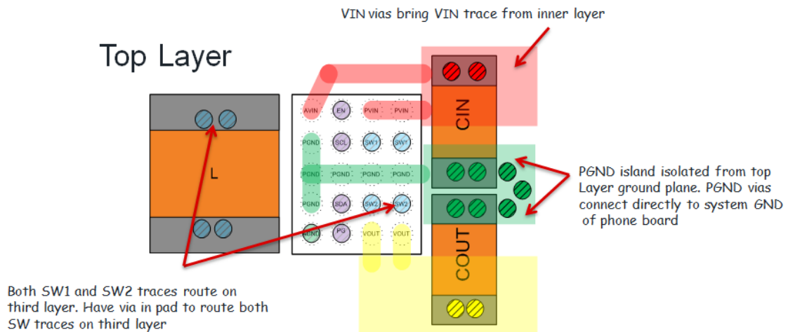
Figure 40. Top Layer Routing for FAN49103
