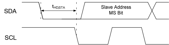
Figure 34. START Bit
