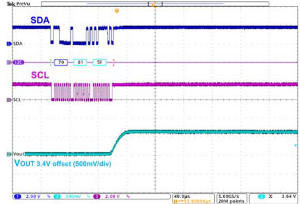
Figure 29. V_{OUT} Transition, 3.4\text{ V} \Rightarrow 4.0\text{ V} , 500 mA Load
