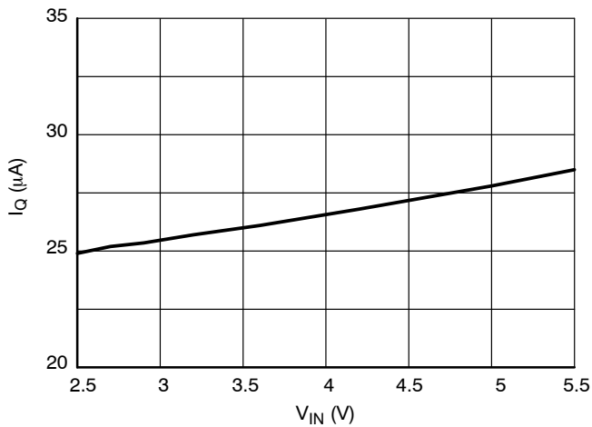
Figure 5. Quiescent Current vs. Input Voltage ( EN = \text{High} , Open Loop, V_{OUT} = 1.8 V , T_A = 25^\circ C )
